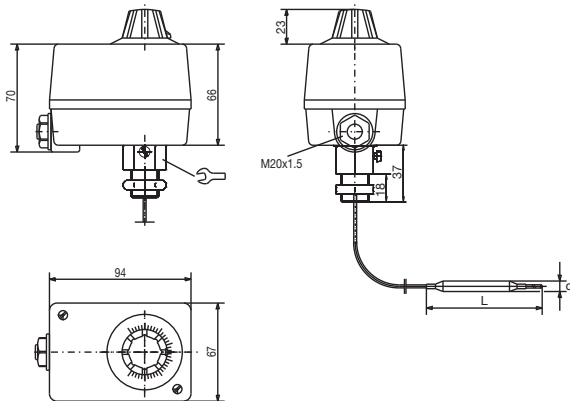
ATH-70, ATH-70/574, process connection "10" plain cylindrical probe
