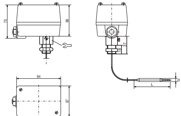
ATH-20/r, ATH-70/r, process connection "42" plain cylindrical probe with weld-in tube G 3/4
