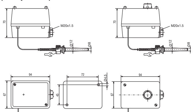
ATH-20/r, ATH-70/r, process connection "42" plain cylindrical probe with weld-in tube G 3/4
