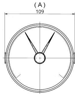
Panel cut-out \varnothing 102^{+0.5}_0 mm
