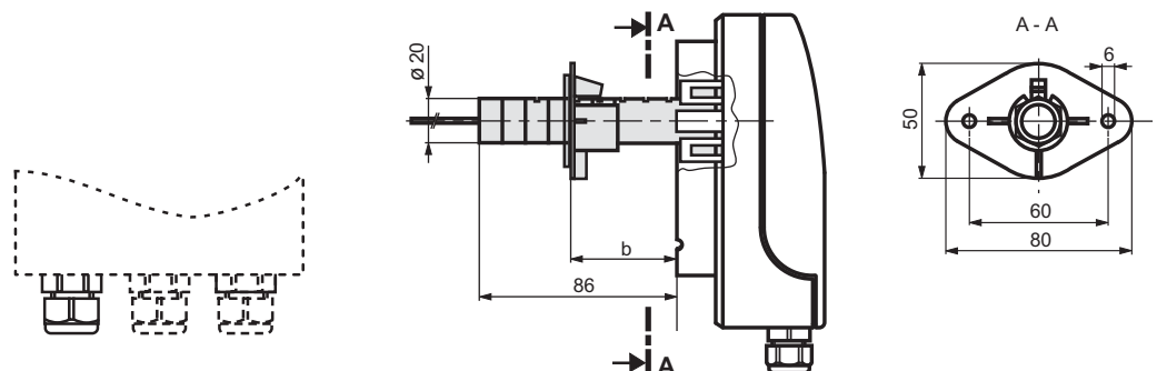
Drilling diagram for direct mounting
