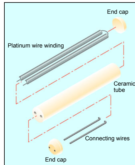
Fig. 10: Basic construction of platinum-ceramic temperature sensors (PK style)
