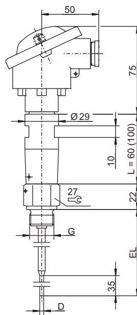
Basic type 902454/11 (DL)
