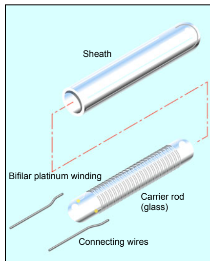
Fig. 7: Basic construction of platinum-glass temperature sensors (PG style)
