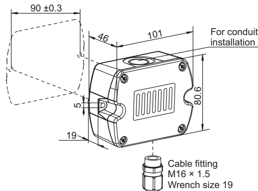
Basic type 907021/820 CO 2 measuring probe, wall-mounted version
