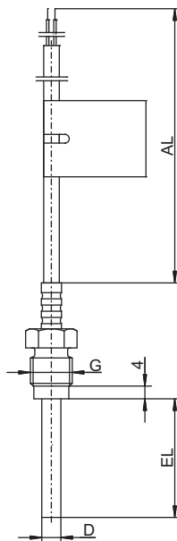
Basic type 902428/40 (DL) Basic type 902455/40 (DL)
