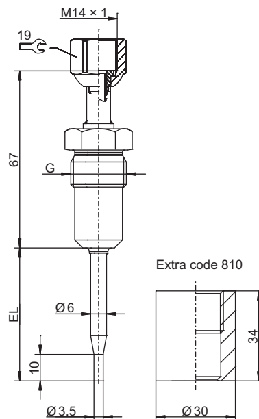
Basic type 902812/10 with process connection PA 380
