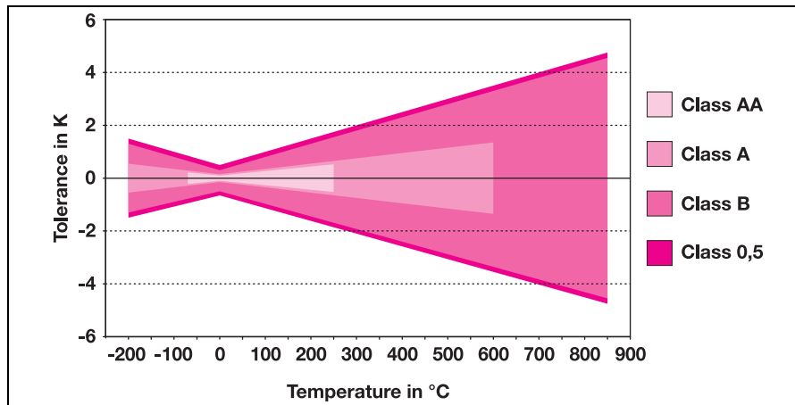
Fig. 2: Tolerance band as a function of the temperature
