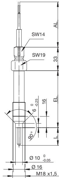
Basic type 901090/50 ... M18 x 1.5
