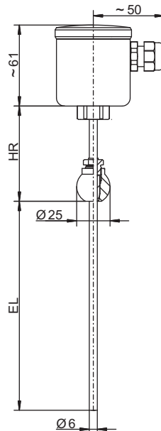
Basic type 902810/20 with process connection PA 681
