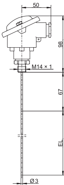
Basic type 902810/40 with process connection PA 120
