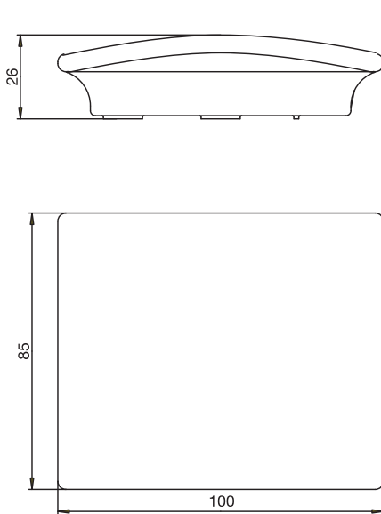
Basic type 907021/11 and 907021/80 indoor version and basic type 907021/12 tabletop and wall-mounted indicator
