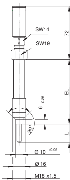
Type 902090/20 ... M 18x1.5
