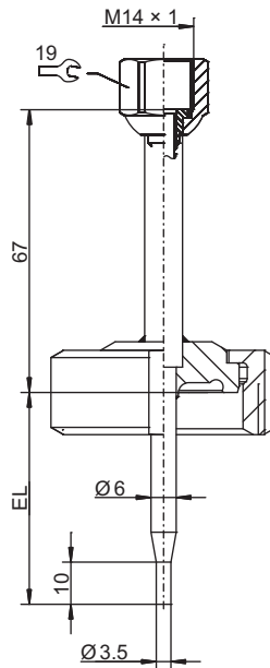
Basic type 902812/10 with process connection PA 550 to 554
