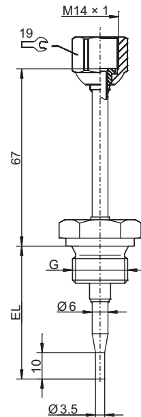
Basic type 902812/10 with process connection PA 104
