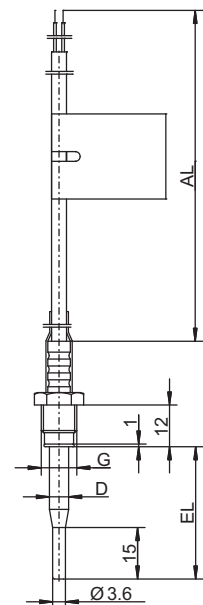
Basic type 902428/70 (DS) Basic type 902455/70 (DS)
