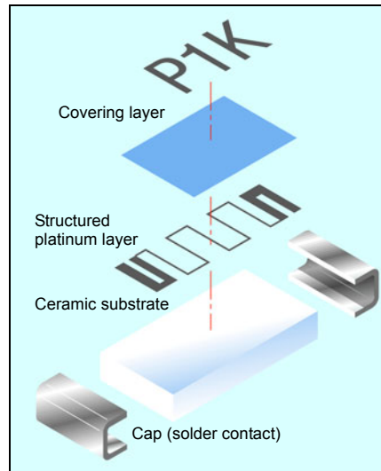
Fig. 16: Basic construction of platinum-chip temperature sensors in SMD style (PCS style)
