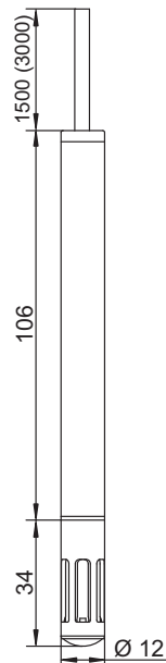
Basic type 907021/60 hygrothermal transducer, rod version with 1.5 m (3 m) connecting cable
