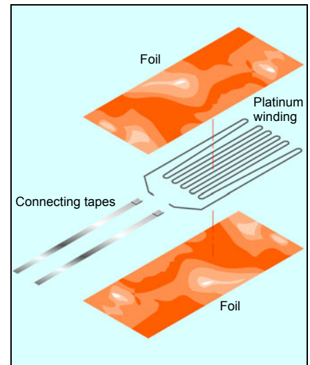
Fig. 11: Basic construction of platinum-foil temperature sensors (PF style)
