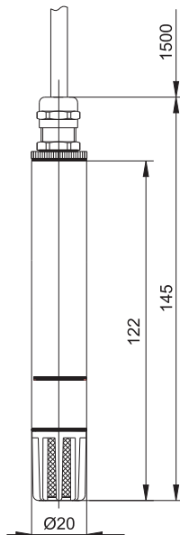
Rod version with connecting cable
