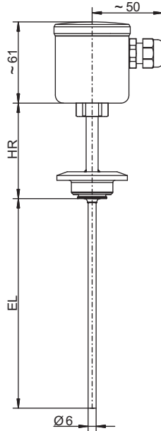
Basic type 902810/20 with process connection PA 684
