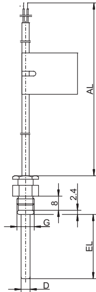
Basic type 902428/50 (DS) Basic type 902455/50 (DS)
