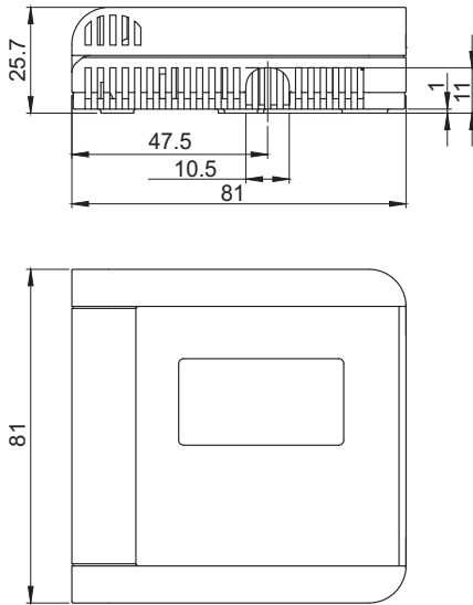
Indoor version (For drilling pattern, see packaging)
