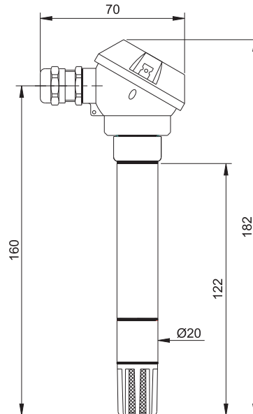
Rod version with form J terminal head
