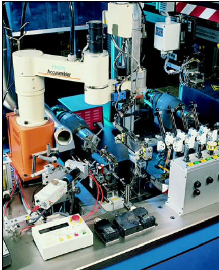
Fig. 9: Automated production of wirewound platinum-glass temperature sensors
