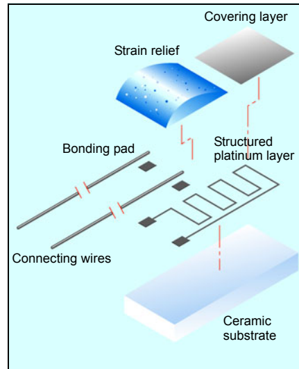
Fig. 13: Basic construction of platinum-chip temperature sensors with connecting wires (PCA style)
