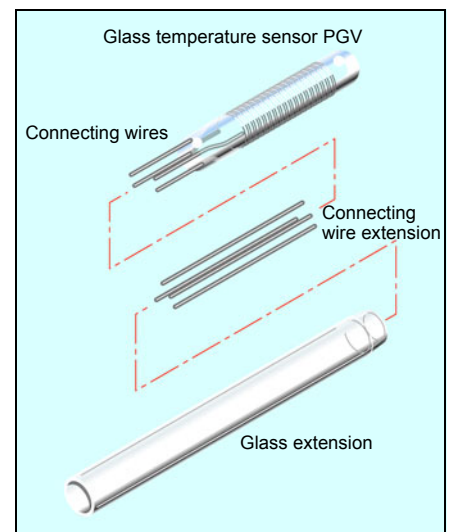
Fig. 8: Basic construction of platinum-glass temperature sensors with glass extension (style for laboratory RTD temperature probes)
