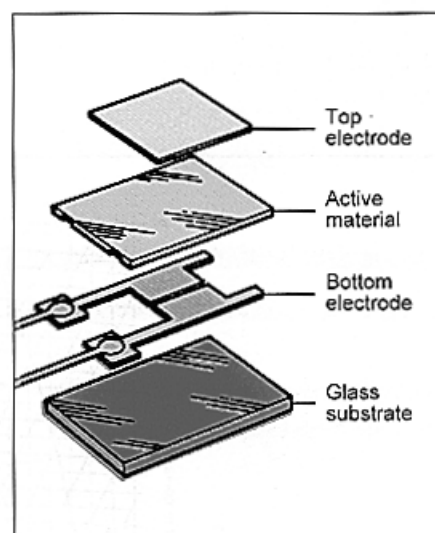
Fig. 5: Construction of the sensor
