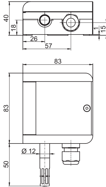
Wall-mounted version (For drilling pattern, see packaging)
